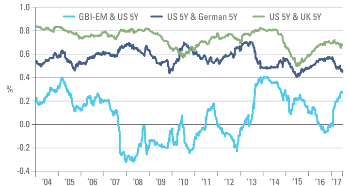
Fig 13: EM rates are less correlated to G7 rates 12-month Correlation of Interest Rates returns (local terms)
